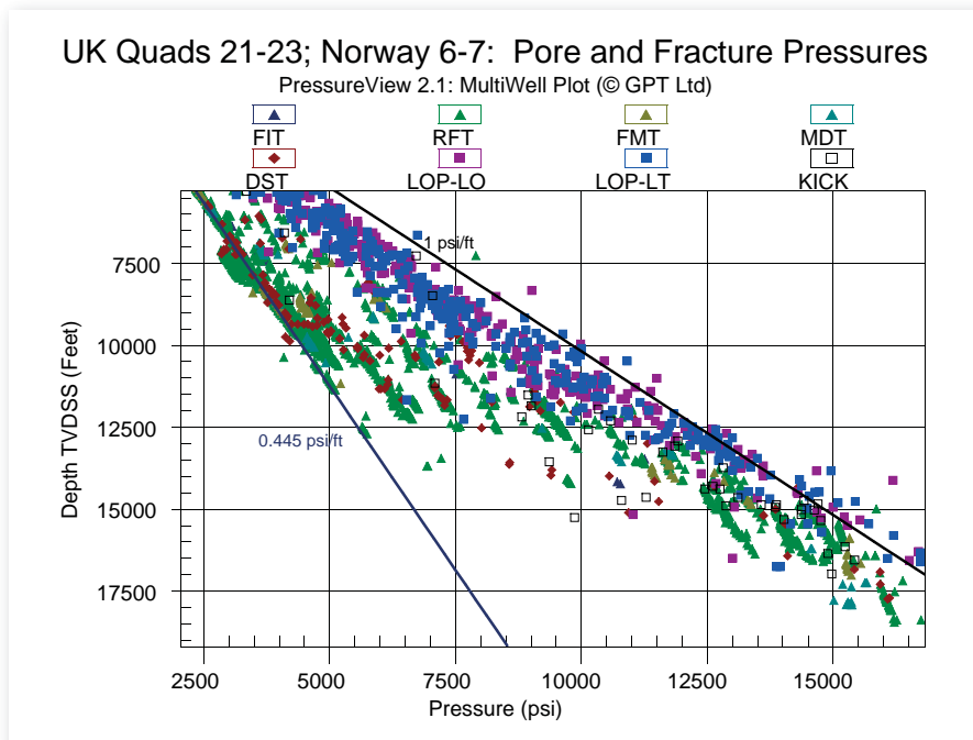
Representative Pressure-Depth Plot 4
